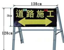
LED 警示拒馬
